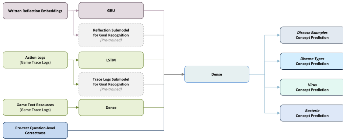
Figure 5. Concept-level stealth assessment model architecture.
