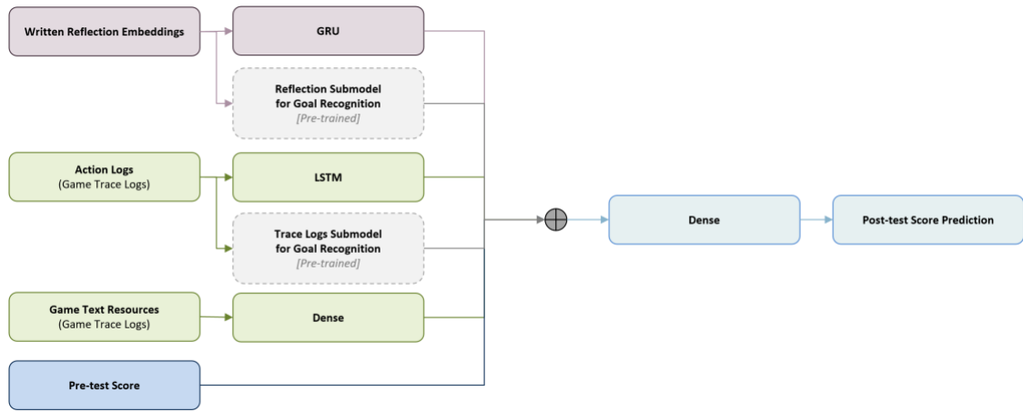
Figure 4. Overall posttest score prediction model architecture.
