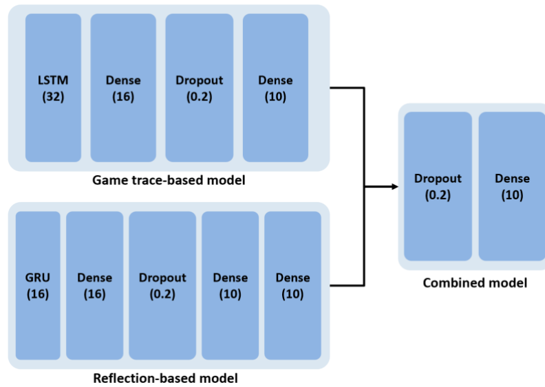
Figure 3. Goal recognition model architecture.
